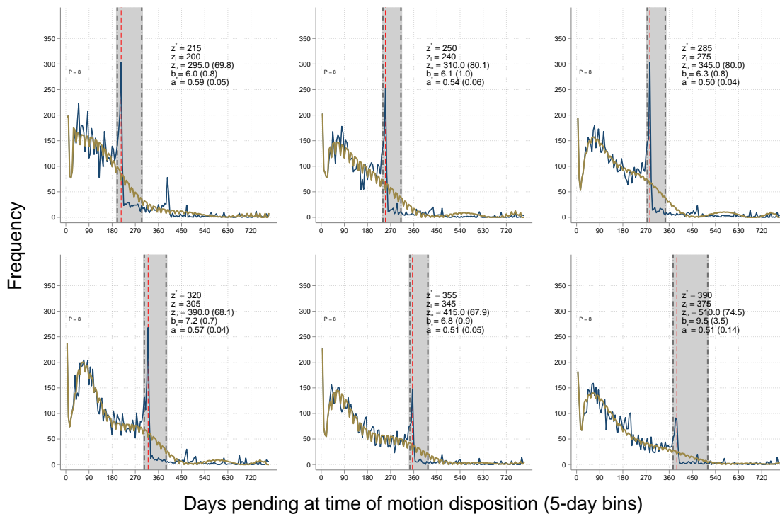
Figure 13: Estimated Bunching and Counterfactual Disposition Times for Six Reporting Time Levels
